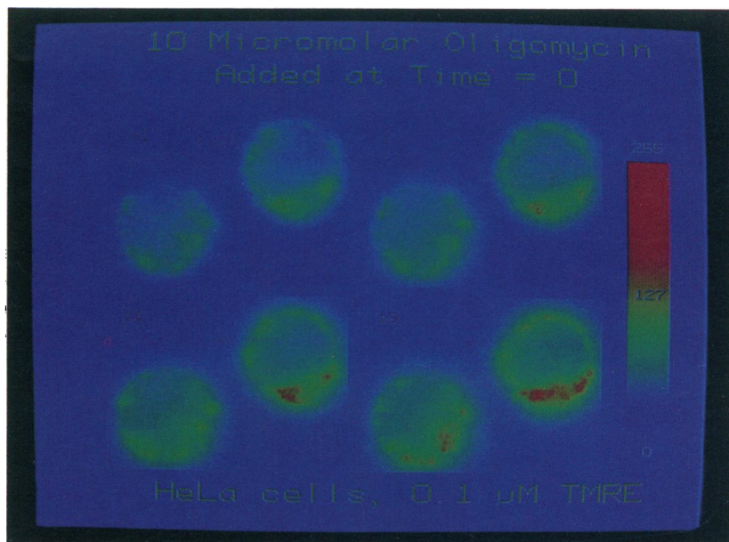
FIGURE 10 Effect of oligomycin on dye fluorescence in cells. HeLa cells incubated in 0.1 \mu M TMRE in EBSS at 22°C were exposed to 10 \mu M oligomycin at time t = 0 . The fluorescence intensities are represented in pseudocolor, with the color scheme shown in the insert. The images correspond to t = -1, 2, 11 , and 19 min. The regions turning from yellow to red after oligomycin addition correspond to the mitochondrial areas.
